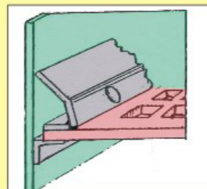
Flat screen deck with support and clamping arrangement
