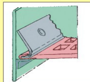
Side longitudinal tensioned screen deck with support and clamping arrangement
