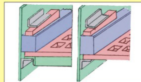
Flat screen deck with side bar and wedge
